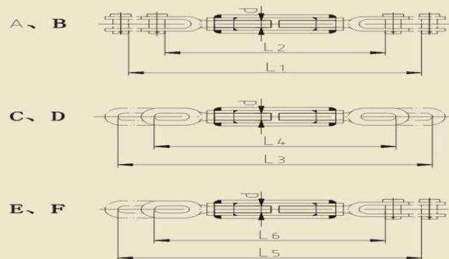
船用开式索具螺旋扣 ( GB561-65 ) TYPE-OPEN TURNBUCKLE FOR SHIP
